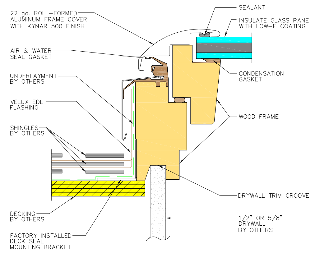
DETAIL 1
