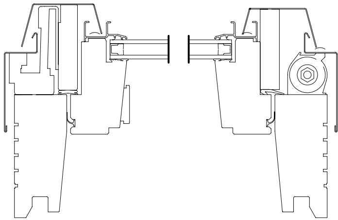
HORIZONTAL CROSS SECTION
