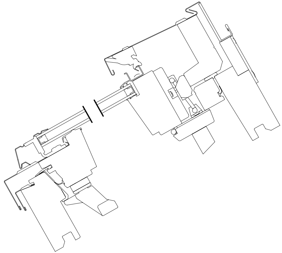
VERTICAL CROSS SECTION
